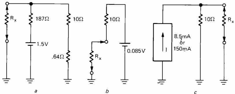
FIG. 10—TWO TYPES OF TEST SIGNAL generators for TVM ohmmeters. Battery and voltage divider combination is shown in a; equivalent circuit is shown in b. Constant-current generator is shown in c.
