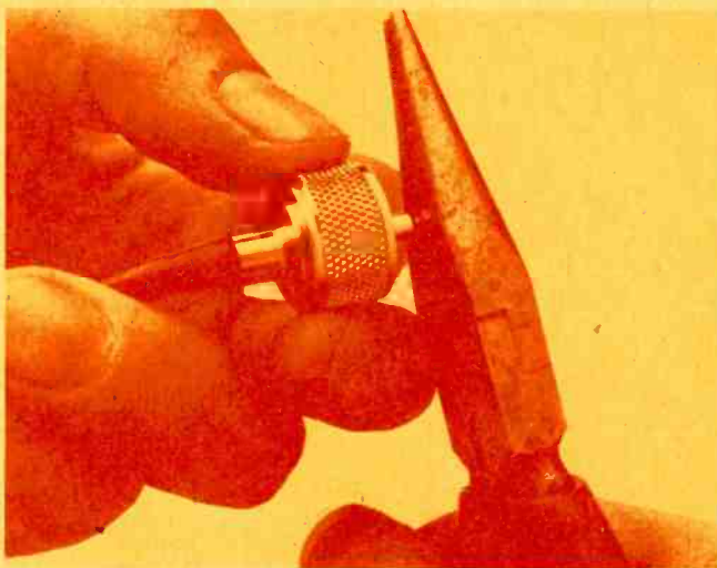
STEP 5—SQUEEZE-CRIMP THE TIP of the center conductor only, with the pliers. If the connector is to be used again, the center contact may be soldered.
