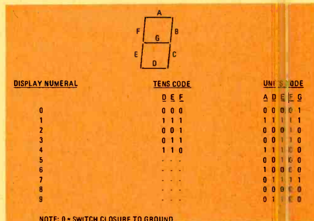
FIG. 5—SWITCH PROGRAMMING of the NC6402 shown in Fig. 4.
