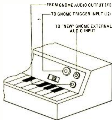
FIG. 11—CONNECTIONS TO GNOME.
