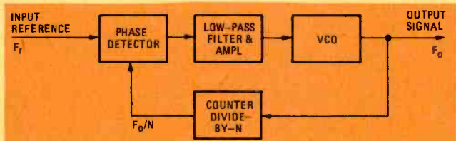
FIG. 2—THE OUTPUT FREQUENCY can be made different from the reference frequency by inserting a divide-by-N counter in the feedback loop. Now the output frequency is equal to N \times F_r .
