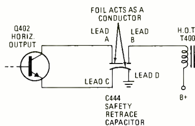
FIG. 5—SAFETY RETRACE CAPACITOR acts as fuse in Sylvania E41, E42 chassis.
