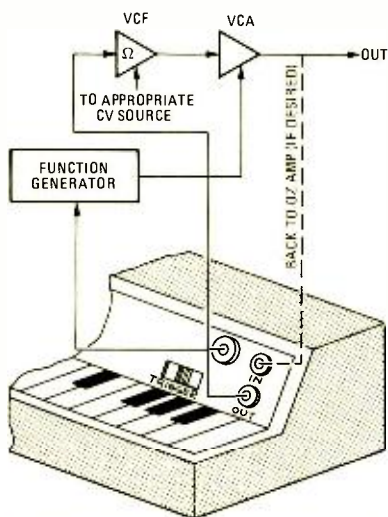
FIG. 9—OZ REPLACES KEYBOARD/VCO.
