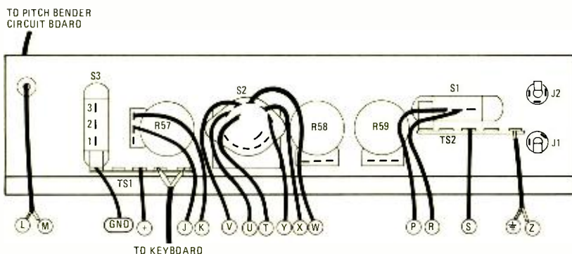
FIG. 6—PANEL-TO-BOARD WIRING.
