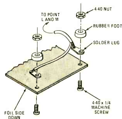
FIG. 7—PITCH-BENDER board assembly.
