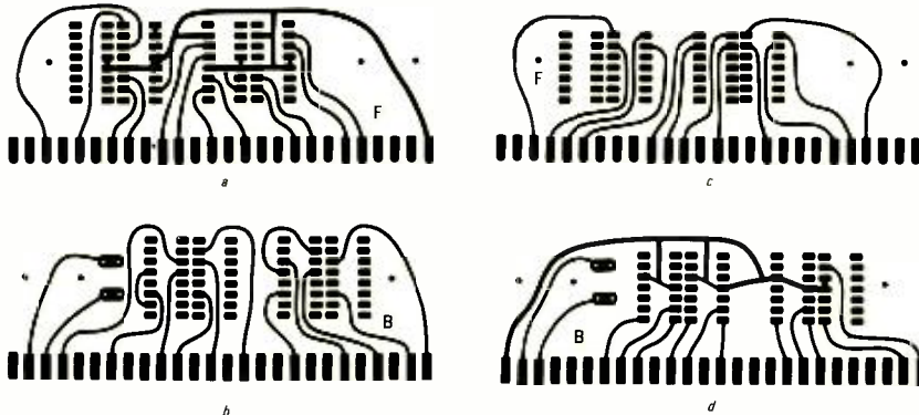
FIG. 7—DISPLAY BOARD foil-patterns shown half-size. a—front of incandescent display board; b—rear of same board; c—front of LED board; d—back of the LED board.
