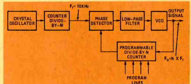
FIG. 3—MULTIPLE OUTPUT FREQUENCIES can be obtained by inserting a programmable divide-by-N counter in the feedback loop. The value of N depends on the data on the program lines.
