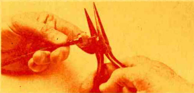
STEP 6—TRIM OFF THE TIP of the coax center conductor to flush it with the barrel.
