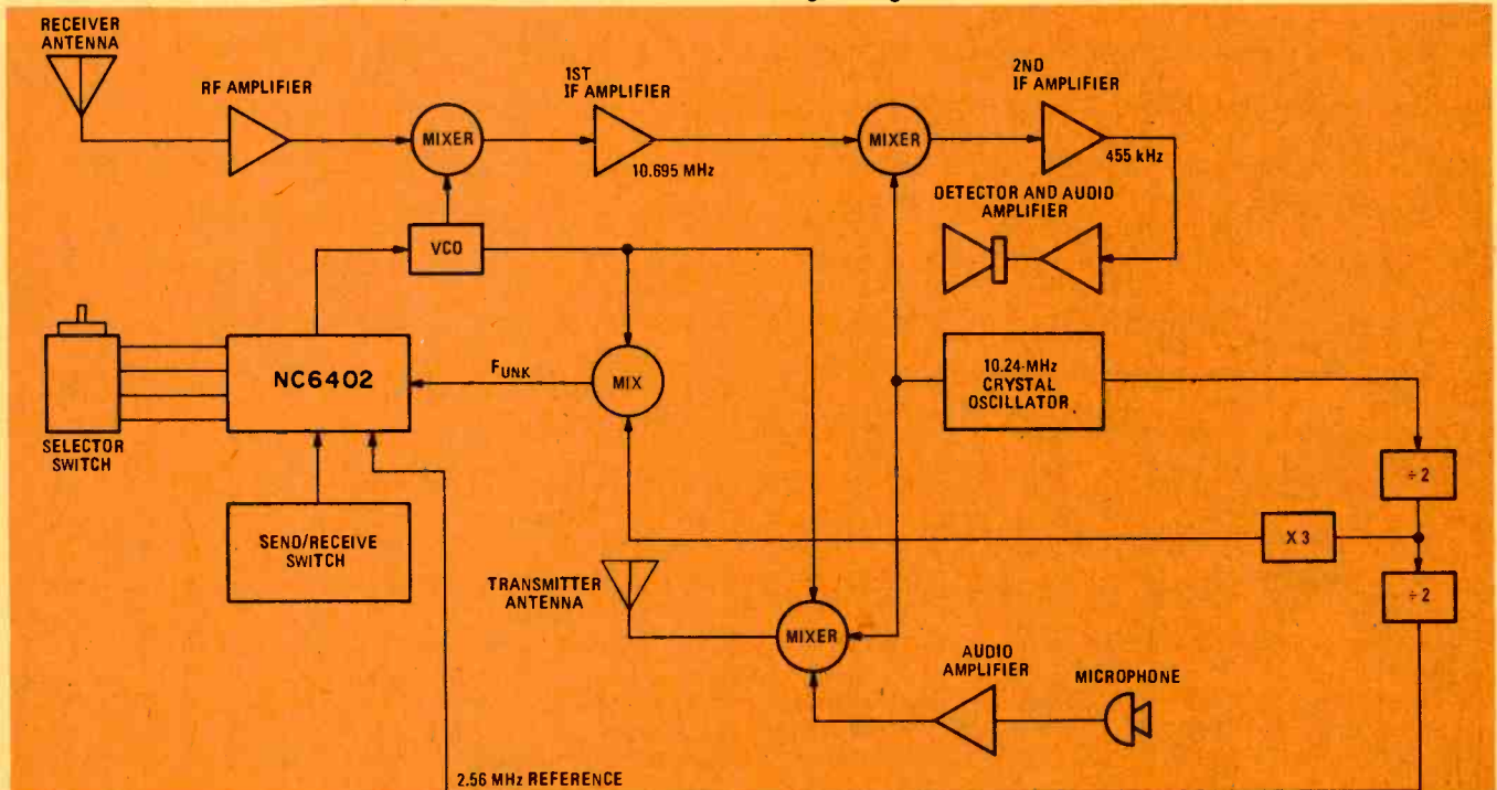
FIG. 4—PLL CIRCUIT of a single-crystal AM CB transceiver.
