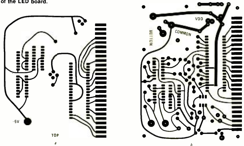
FIG. 10—THE MAIN BOARD foil-patterns shown half-size. a shows component side; b shows bottom. If board is made a little larger, corner holes may be moved out slightly; they are now positioned for minimum-sized board.
