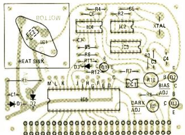
FIG. 11—COMPONENTS LAYOUT, MAIN CIRCUIT BOARD. Top view. Capacitor C2 mounts to bottom of board. Unless pins of MM5385 and 74C221 are bent back 180 degrees (see text) they must also be mounted to bottom of board.
