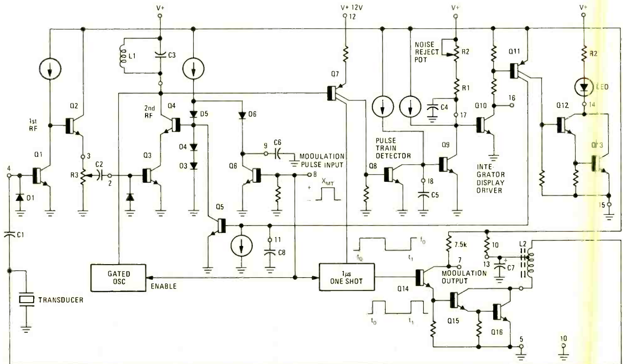
FIG. 1—NATIONAL SEMICONDUCTOR LM1812 ULTRASONIC TRANSCIEVER.
