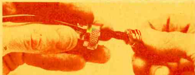
STEP 3—POSITION THE BODY so the braid flattens against its rear flange.
