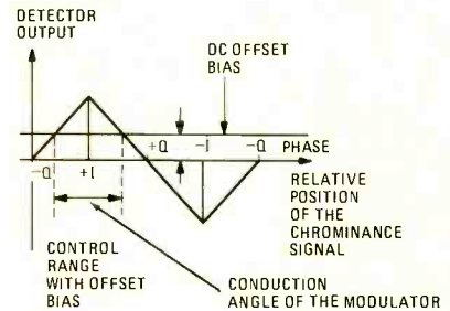
FIG. 2—OFFSET BIAS CONFINES color correction to colors near flesh tones.
