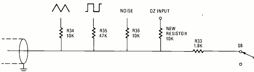
FIG. 10—THE GNOME'S AUDIO BUS, showing the added input and 10K resistor.
