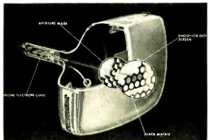
THE GENERAL ELECTRIC 25-inch in-line color picture tube.
