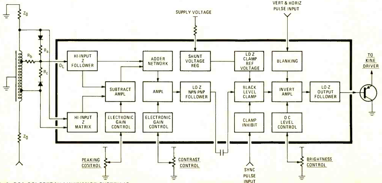
FIG. 3—RCA COLORTRAK LUMINANCE SYSTEM IC.
