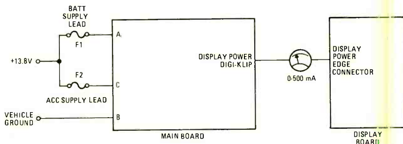
FIG. 12—CALIBRATION SETUP. Install both fuses before turning on power; set both pots to minimum resistance. If displays show an illegal readout after clock has been reset at initial power turn-on, disconnect power and troubleshoot the display board and displays for shorts or opens. Voltages shown are for a 12-volt system, engine running.
