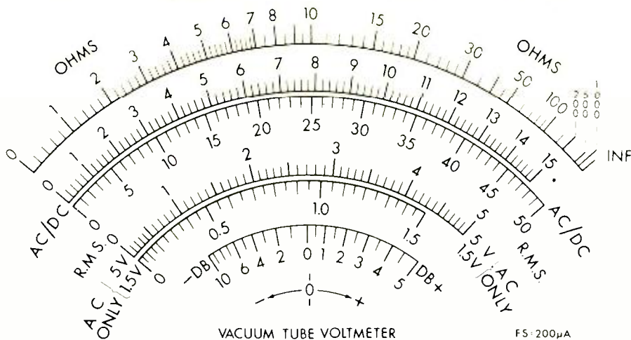
FIG. 11—A TYPICAL VTVM SCALE. Center-scale reading is 10 ohms or a multiple; non-linearity is well shown. Note the special low-voltage scales for AC.
