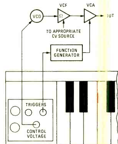
FIG. 8—A SYNTHESIZER PATCH. The initials stand for voltage controlled oscillator, filter, amplifier, and control voltage source.
