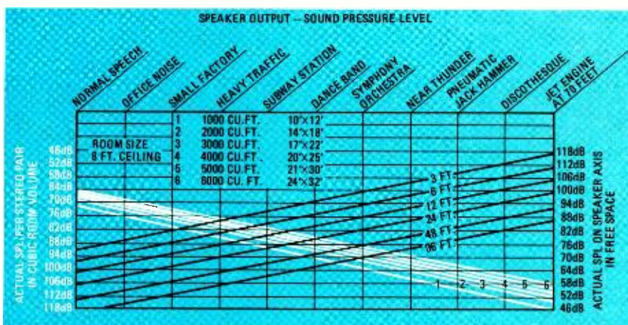
FIG. 5—GRAPH ON FRONT-PANEL enables user to translate power readings into actual sound pressure levels.
