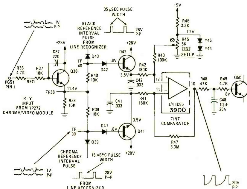
FIG. 4—GENERAL ELECTRIC VIR TINT COMPARATOR.
