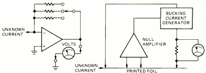
FIG. 9—TWO SPECIAL CIRCUITS for measuring current. Operational amplifier used as current-to-voltage converter is shown in a. Ranges are selected by the feedback resistor. The patented Weston circuit that sets up a bucking current equal to the unknown one and then measures the bucking current is shown in b.
