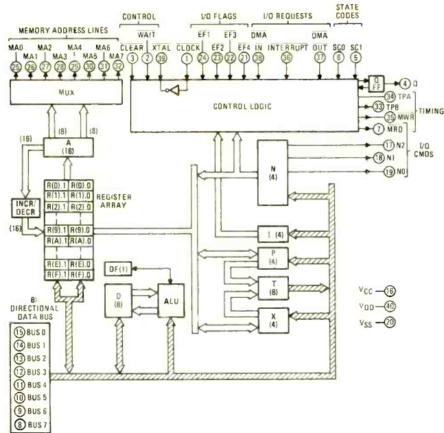
FIG. 2—BLOCK DIAGRAM OF THE RCA CDP1802.
