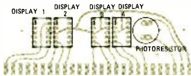
FIG. 8—DISPLAY BOARD COMPONENTS LAYOUT. Front view. Bezel mounting holes are centered by drawing a line across board, through the center of the displays. Inner bezel holes accommodate Allied 658-1240 bezel; outer ones the 658-1260. The photoresistor mounting holes are for Archer 276-116 or Clairex CL704L. Photoresistor solder pads are large enough to accommodate Clairex CLM54L if Allied 658-1260 bezel is used.
