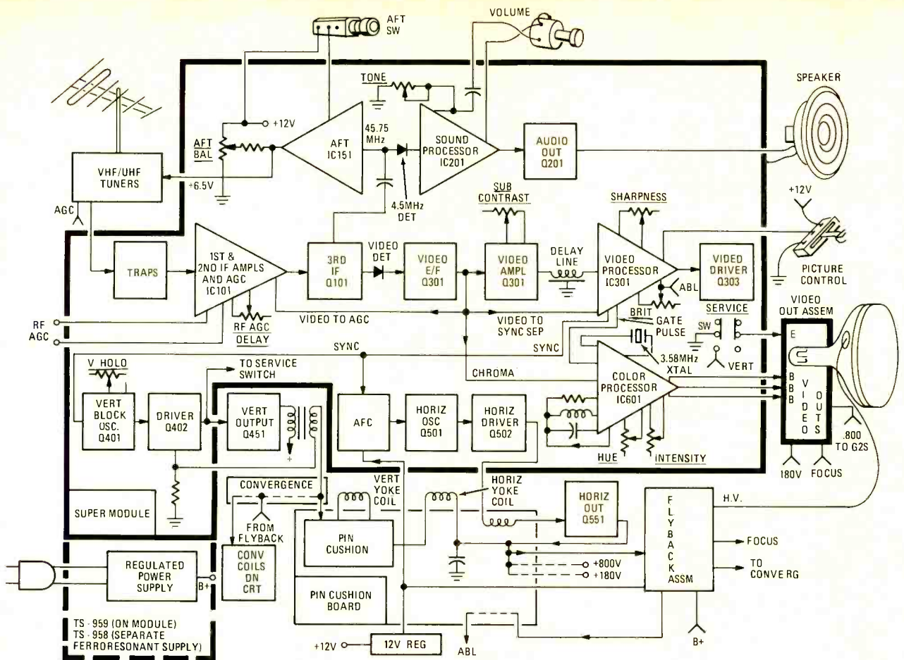
FIG. 1—BLOCK DIAGRAM, QUASAR TS958/959, showing Super Module.
