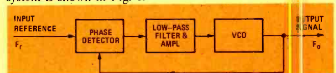
FIG. 1—SIMPLE PLL CIRCUIT produces an output frequency equal to the input reference frequency.
